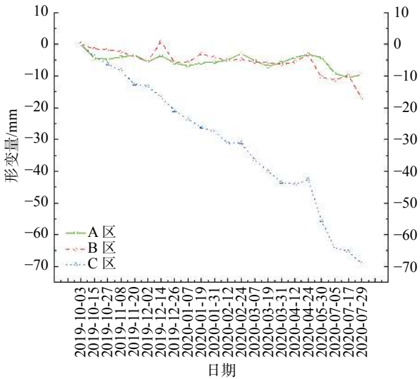
图 3 绞东滑坡三处斜坡区平均形变时序曲线图 Fig. 3 Time series curve of average deformation in three slope areas of Jiaodong landslide
