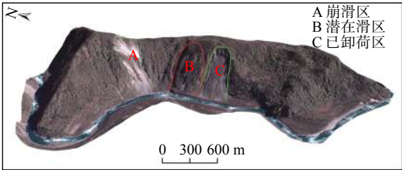
图 2 绞东滑坡斜坡区三维影像图 Fig. 2 3D image of Jiaodong landslide slope area
