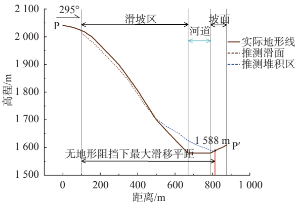
图 5 绞东滑坡潜在滑区(B 区)地形剖面示意图 Fig. 5 Topographic profile of potential sliding area(B) of Jiadong landslide
