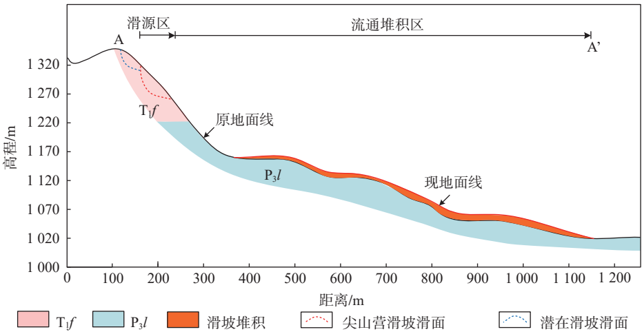
图 3 尖山营滑坡剖面图(A-A'剖面) Fig. 3 Longitudinal cross-section geological profile of the Jianshanying landslide (section A-A')
