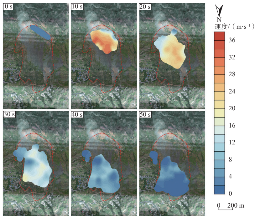
图 7 尖山营滑坡-碎屑流运动过程不同时刻速度分布云图 Fig. 7 Cloud map of velocity distribution of the landslide-debris flow movement in the Jianshanying landslide at different moments
