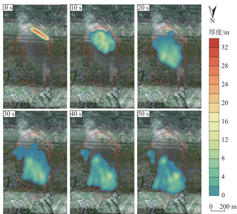
图 6 尖山营滑坡-碎屑流运动过程不同时刻滑体堆积形态 Fig. 6 Landslide accumulation distribution patterns for landslide-debris flow deposits of the Jianshanying landslide at different moments
