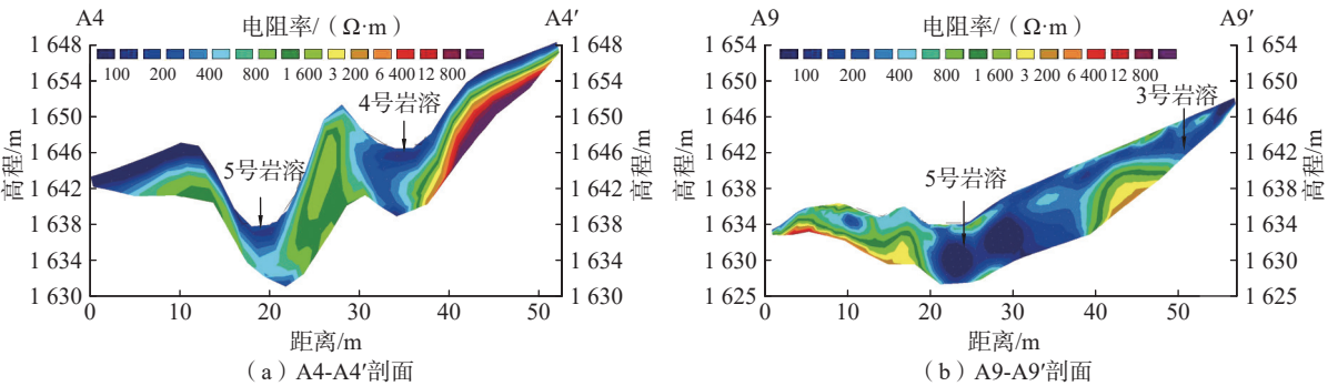
图 3 高密度电法剖面图 Fig. 3 Profiles determined by high-density electrical technique
