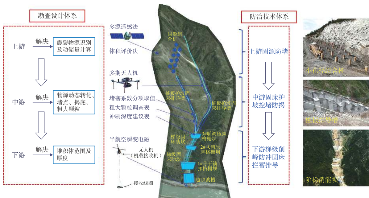
Fig. 6 Schematic diagram of the comprehensive control system for narrow and steep debris flow
