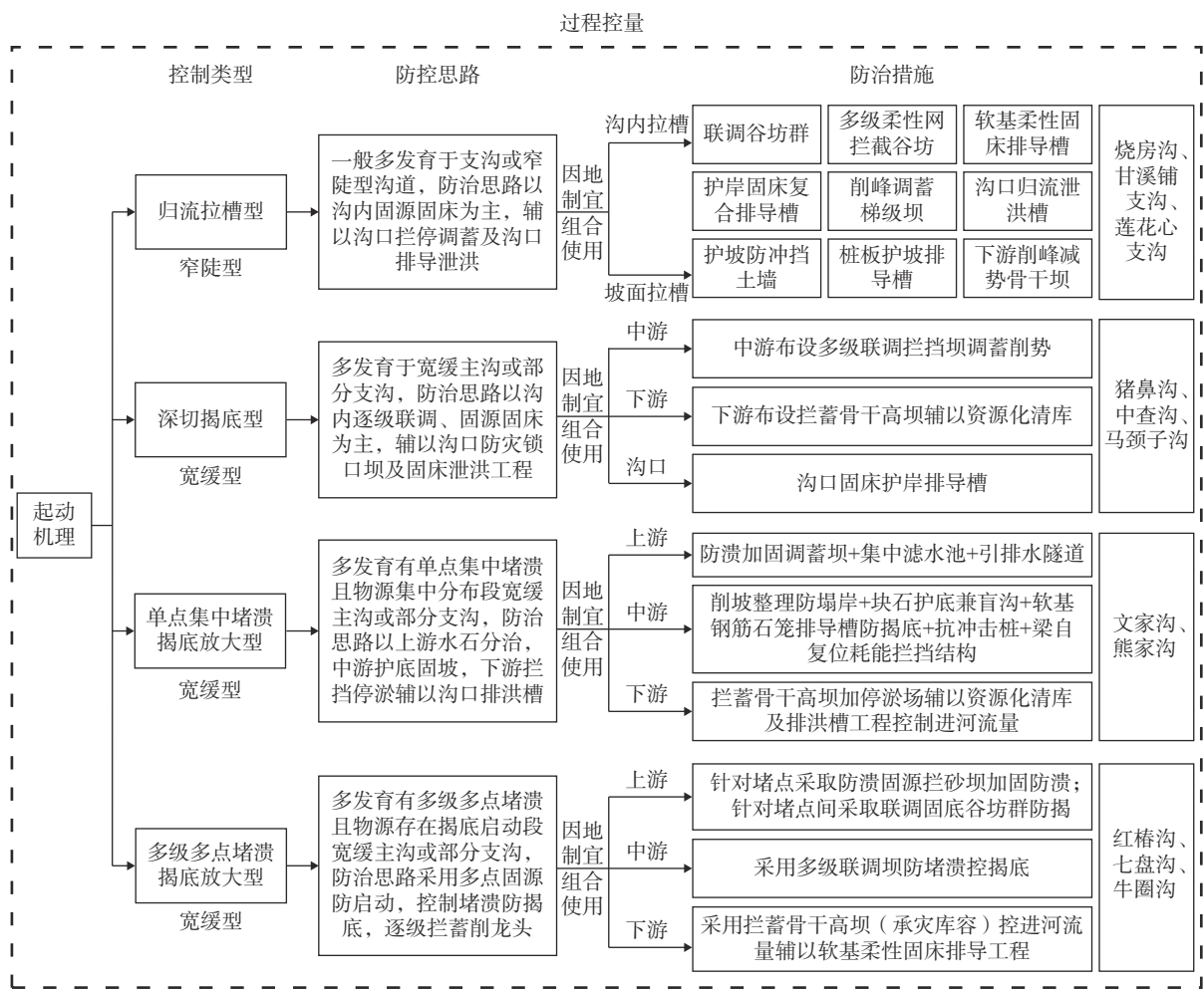
图 4 “过程控量”关键技术体系框架图 Fig. 4 Framework diagram of the key technology system of “Quantity control during the process”
